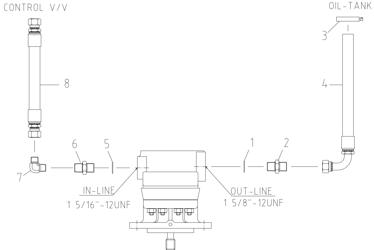
Fig. 8-5 SCS514SL M / T PIPING PART
