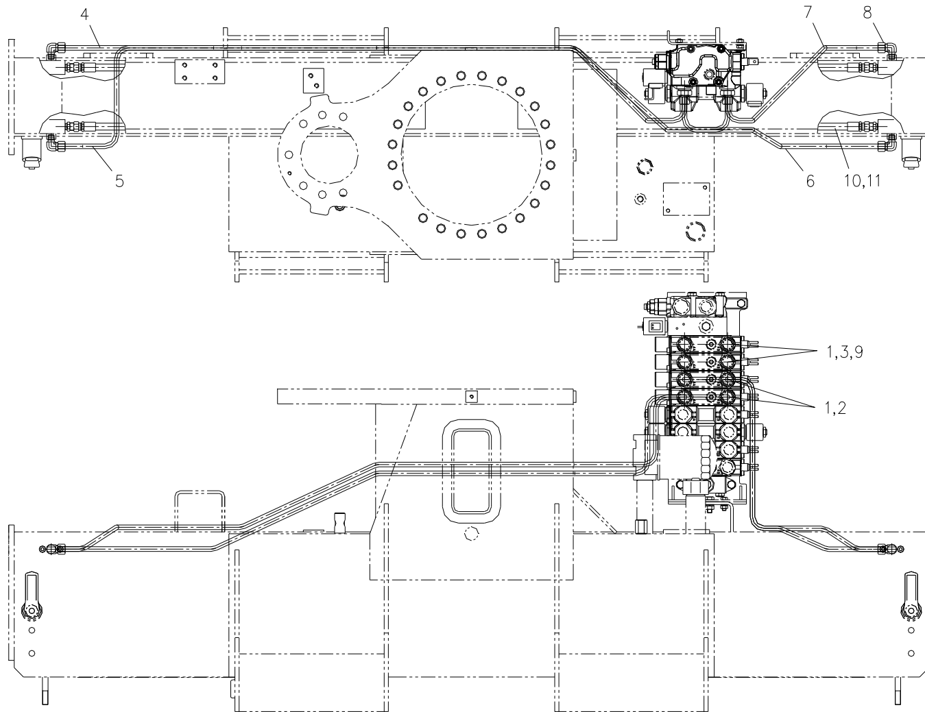
Fig. 5-6 SCS514SL OUTRIGGER PIPING
