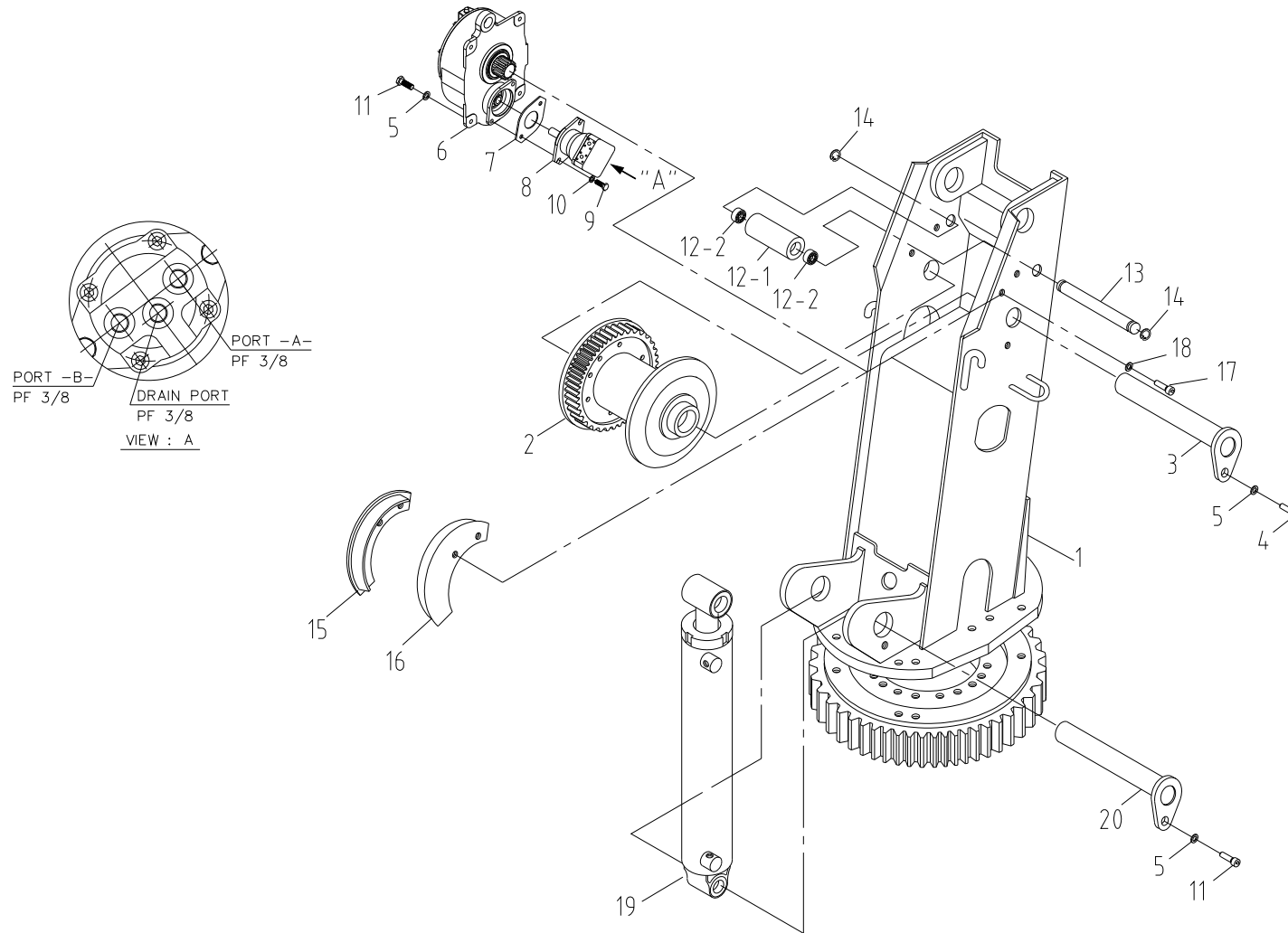
Fig. 2 SCS514SL SWING POST ASS'Y
