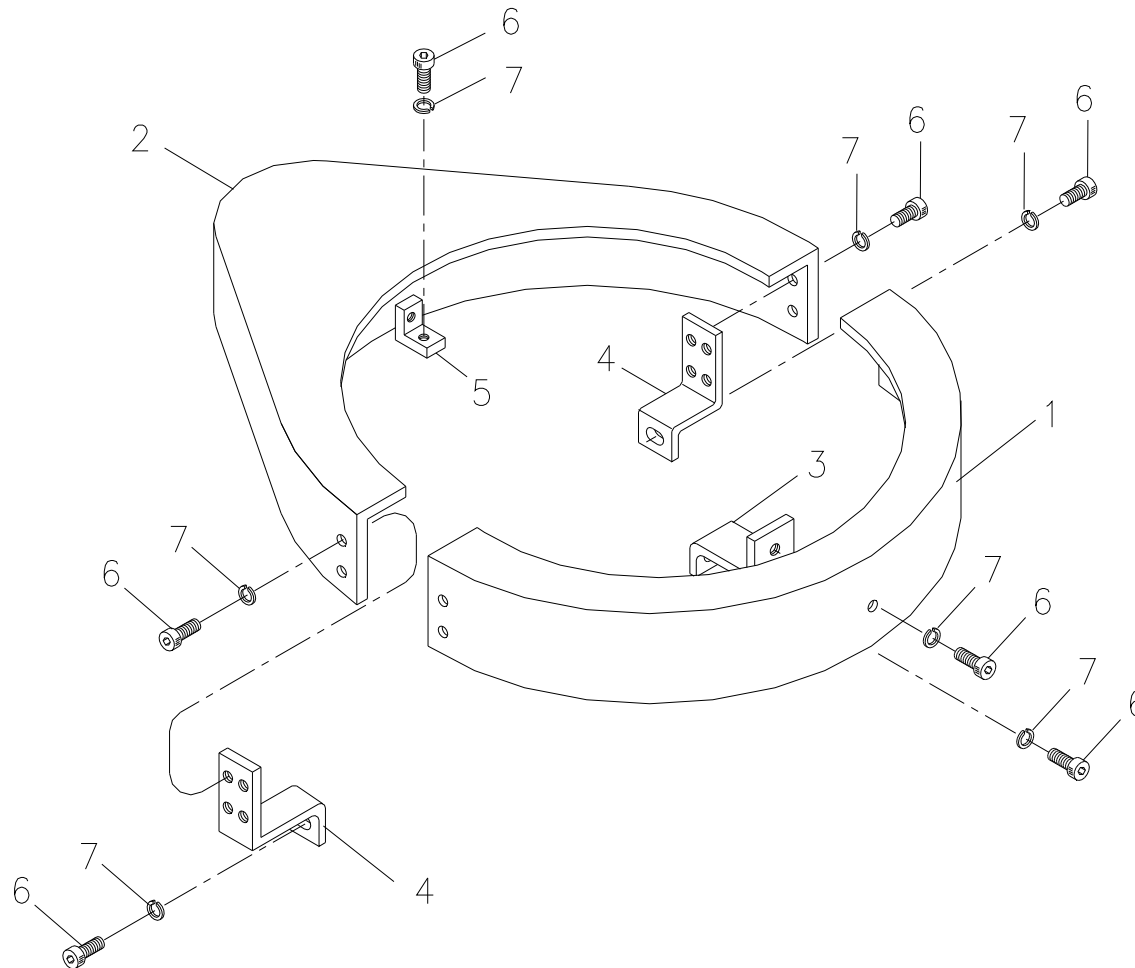
Fig. 3-5 SCS514SL SWING COVER ASS'Y
