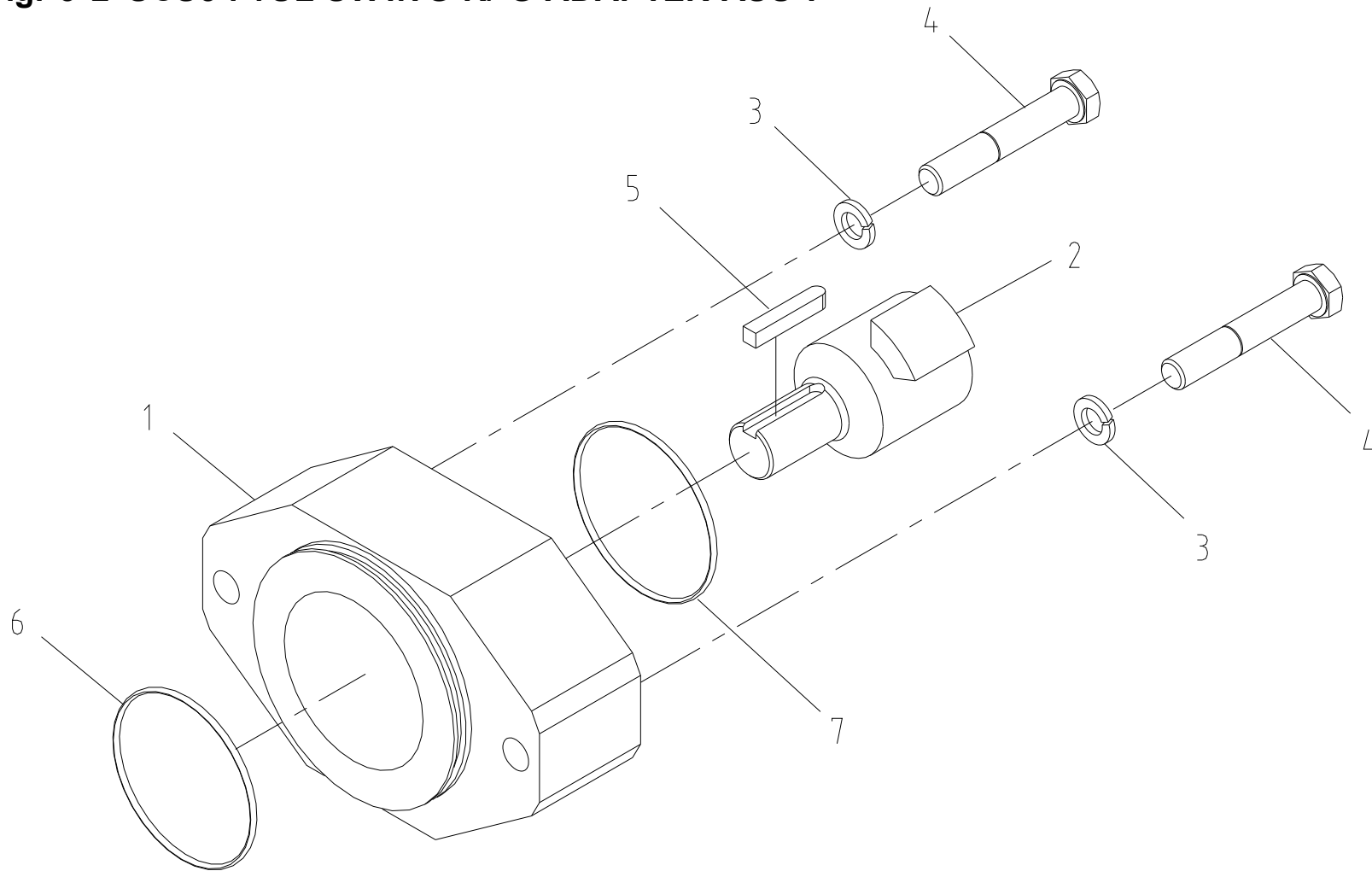
Fig. 3-2 SCS514SL SWING R/ G ADAPTER ASS'Y
